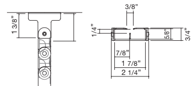
Cable Guard Dimensions
