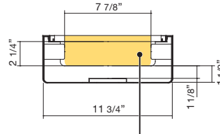
Wiring Duct Joint Part Dimensions
