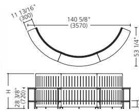
Convex R type shelf set w/panel
